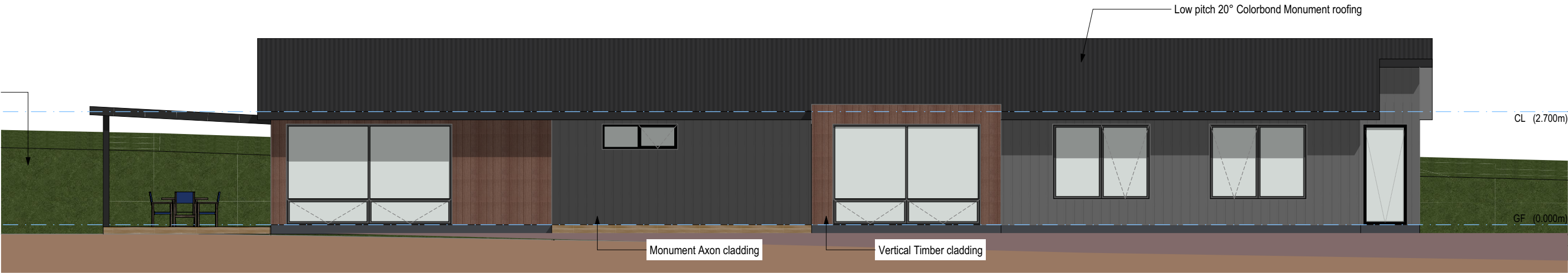
WEST ELEVATION 1:100
