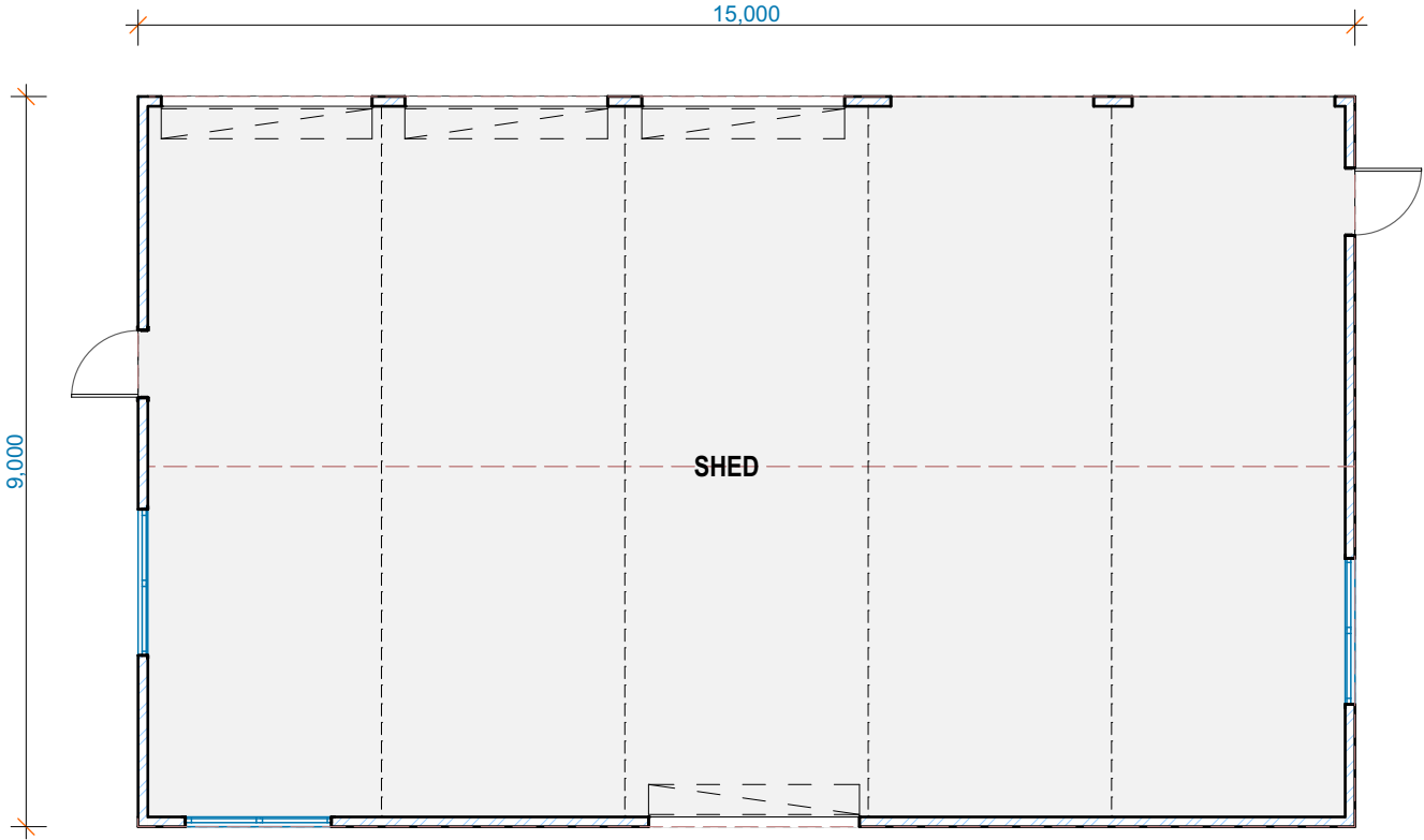
SHED FLOOR PLAN 1:100
