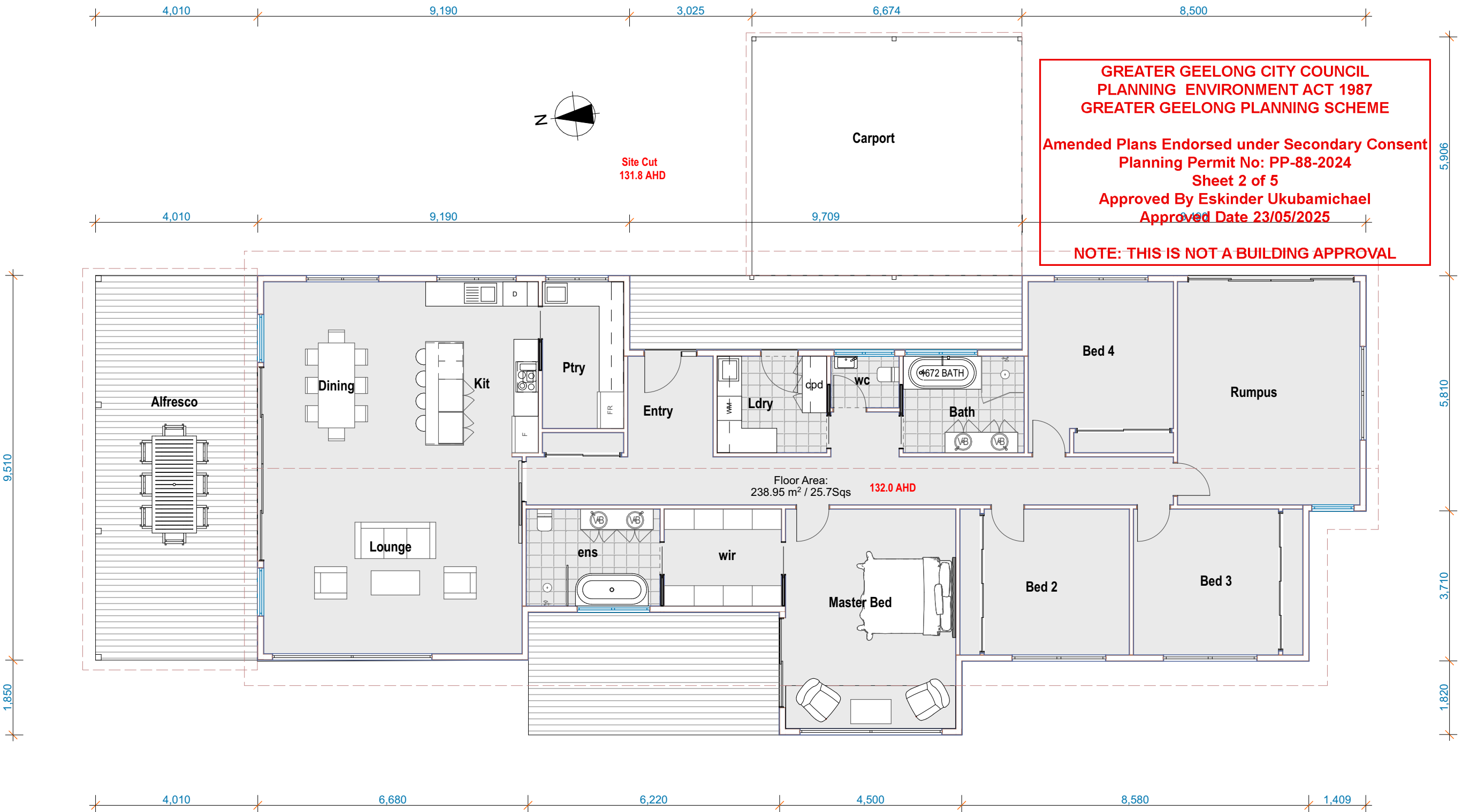
GROUND FLOOR 1:100
